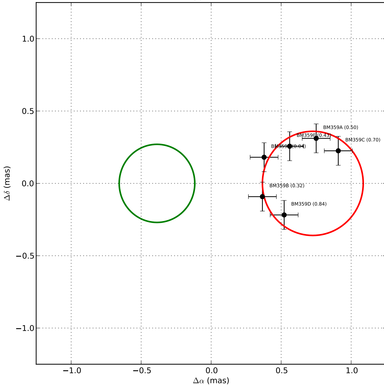
Radio centroids w.r.t. corotating position \rho = 0.6 mas, \phi_0 = 99.3 deg
